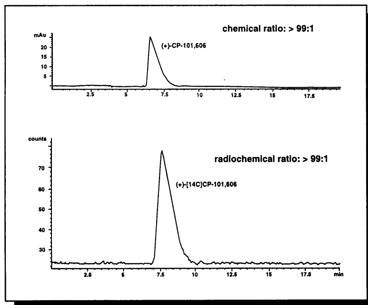
Figure 3. (+)-[ 14 C]CP-101,606 after the final recrystallization.
